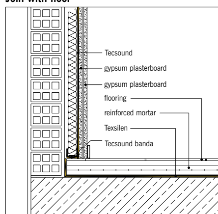
Join with floor
